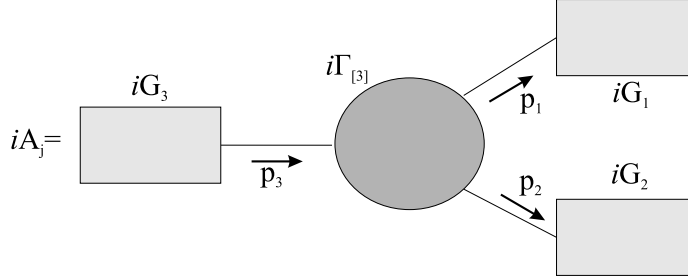
Fig. 1. Feynman diagram for amplitude A_j
