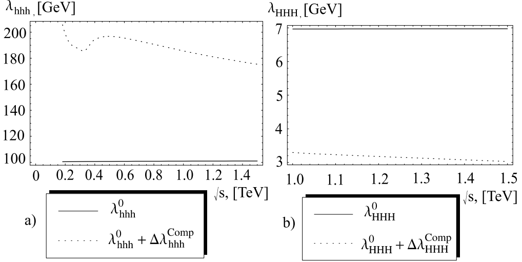
Fig. 4. Dependence of the trilinear Higgs self-couplings (on the tree and one-loop levels) on \sqrt{s} , for \tan\beta = 30 , M_A = 500 GeV, M_3 = \mu = 300 GeV, M_{\tilde{Q}} = M_{\tilde{U}} = M_{\tilde{D}} = M_{\tilde{R}} = M_{\tilde{L}} = 1 TeV, A_f = 200 GeV
