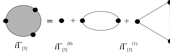
Fig. 2. Vertex function decomposition: the one-loop approximation
