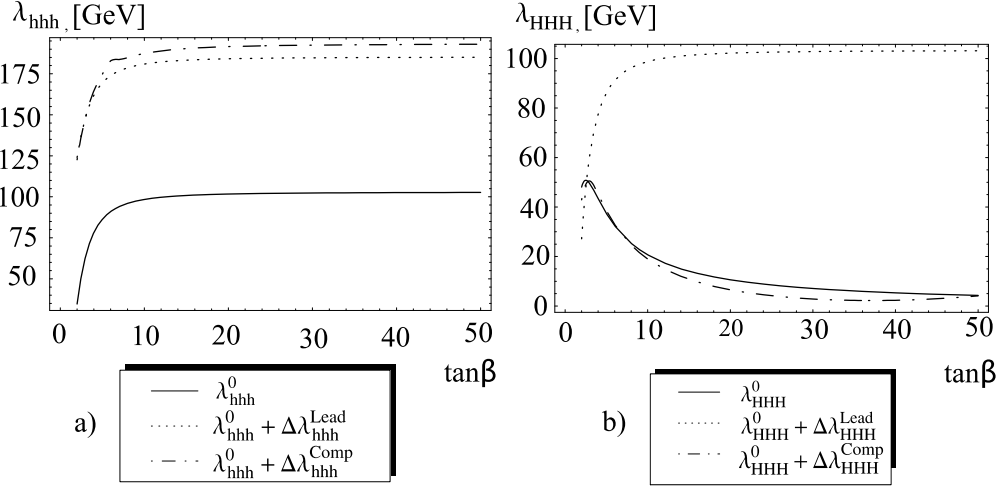
Fig. 3. Dependence of the trilinear Higgs self-couplings (on the tree and one-loop levels) on \tan\beta , for \sqrt{s} = m_{Hg_1} + m_{Hg_2} + 10 GeV, M_A = 500 GeV, M_3 = \mu = 300 GeV, M_{\tilde{Q}} = M_{\tilde{U}} = M_{\tilde{D}} = M_{\tilde{R}} = M_{\tilde{L}} = 1 TeV, A_f = 200 GeV
